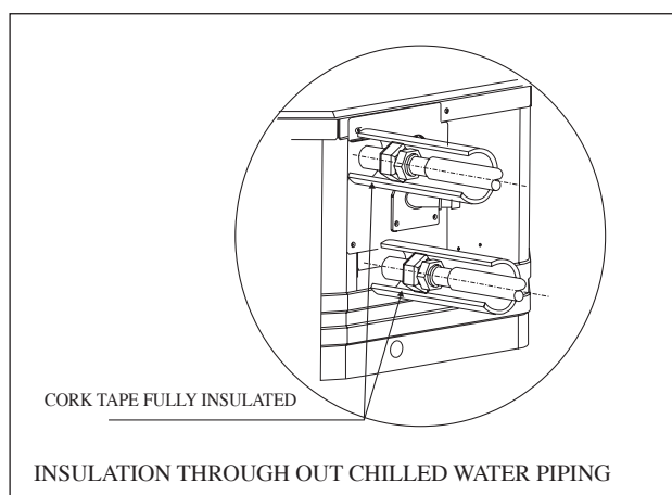
2 Pipes System
