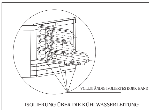
4 Rohre System
